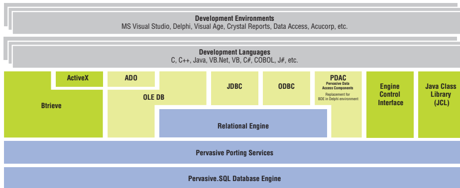
Fig. 1: The Pervasive PSQL Architecture
