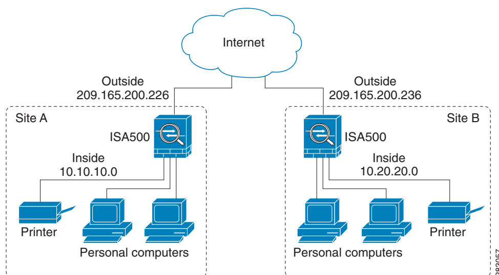
Figure 3 Site-to-Site VPN
